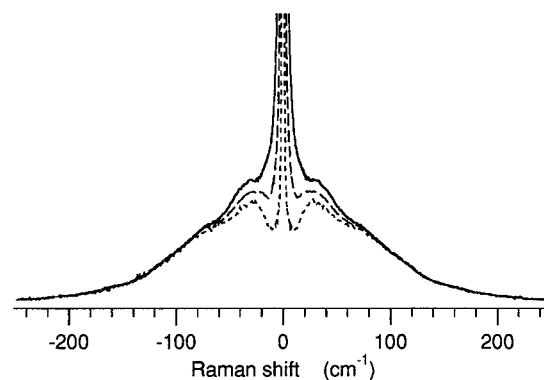
FIGURE 4 Raman spectra I_s(\omega) of wet, semidry, and dry lysozyme crystals in the x(zx)z geometry. The solid line, dashed line, and dotted line correspond to wet, semidry, and dry crystals, respectively.
