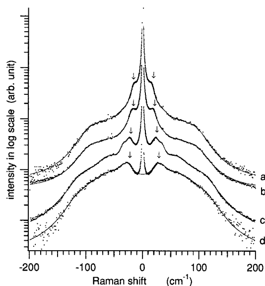
FIGURE 6 Raman spectra I_s(\omega) of DNA films with various water contents on a log scale. The dots and solid lines represent measured and fitted spectra, respectively. The S mode is indicated by arrows. ( a ) B form DNA at 100% r. h. ( b ) B form DNA at 95% r. h. ( c ) A form DNA at 75% r. h. ( d ) disordered DNA.
